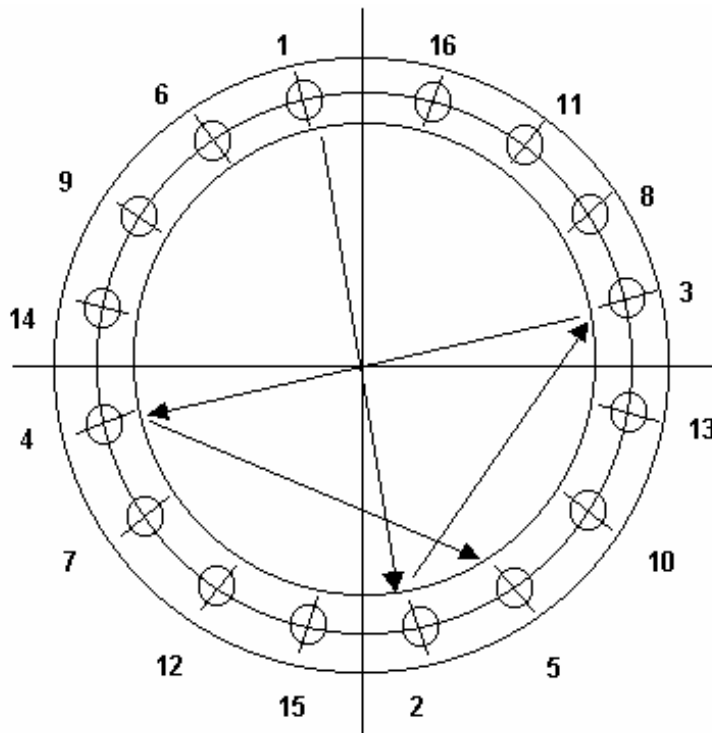
Figure 2: (Un-)bolting sequence
