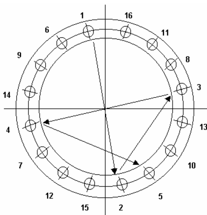
Figure 2: (Un-)bolting sequence
