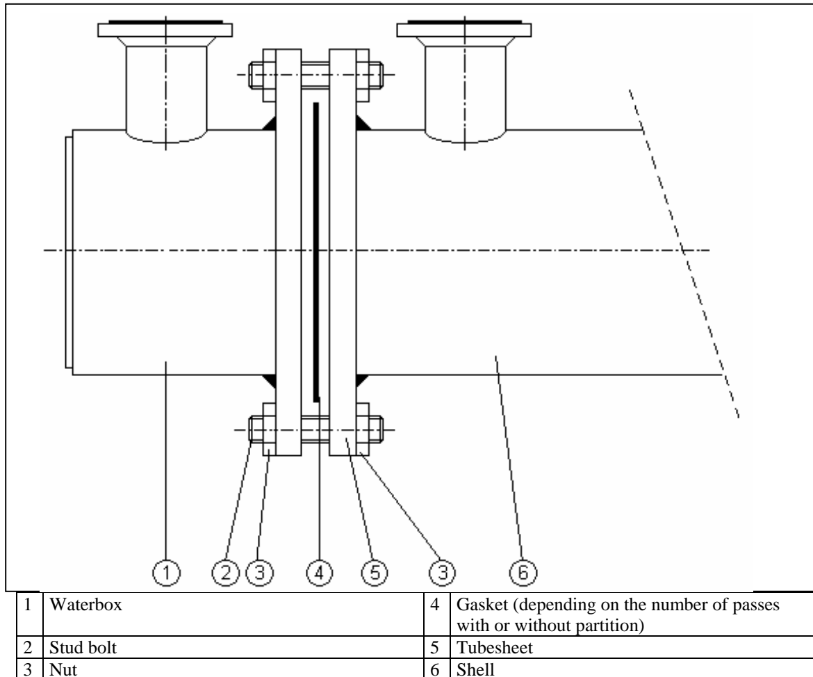
Figuur 1: Schematic drawing of tubesheet construction
